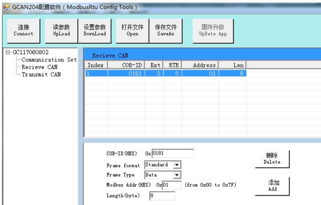
图 4.6 Receive CAN 映射设置
