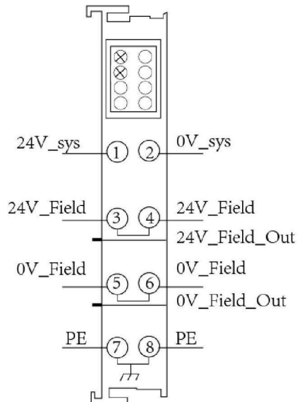
Figure 2.8 GCAN-PLC-511, Power terminal block
